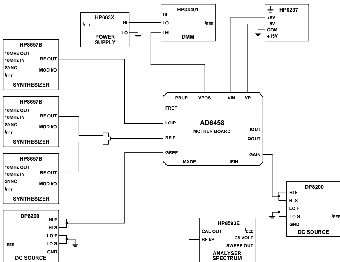
Figure 3. Mixer Characterization Setup
