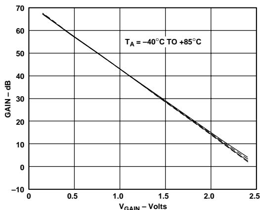
Figure 13. IF Amplifier and Demodulator Gain vs. V_{GAIN} , T_A = +25^\circ C , V_{POS} = 3.0 V , F_{IF} = 13 MHz , V_{REF} = 1.2 V
