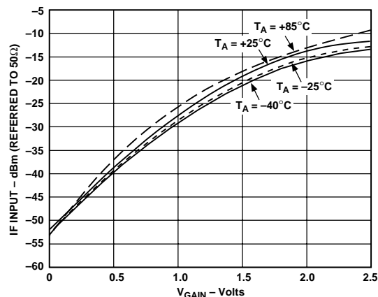
Figure 14. IF Amplifier/Demodulator Input 1 dB Compression Point vs. V_{GAIN} , F_{IF} = 13 MHz , V_{REF} = 1.2 V , T_A = +25^\circ C , V_{POS} = 3.0 V
