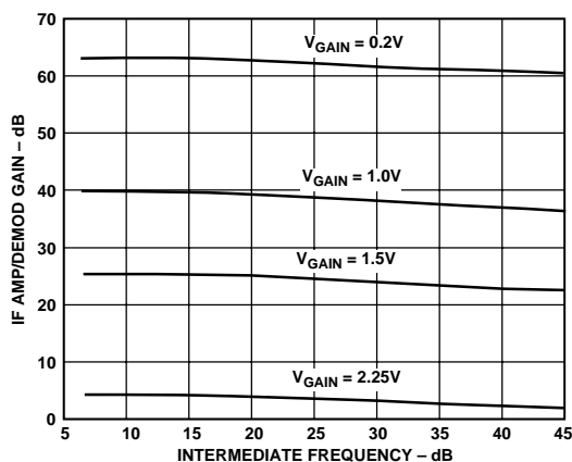
Figure 12. IF Amplifier and Demodulator Gain vs. Frequency, T_A = +25^\circ C , V_{POS} = 3.0 V , V_{REF} = 1.2 V
