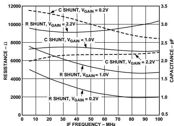
Figure 15. IF Amplifier Input Impedance vs. Frequency, T_A = +25^\circ C , V_{POS} = 3.0 V , V_{REF} = 1.2 V
