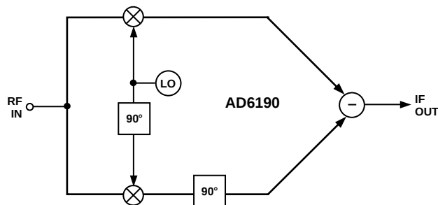
Figure 9. Image-Reject Mixer
