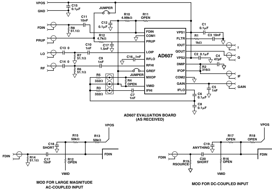
Figure 45. Evaluation Board
