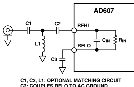
Figure 33. Mixer Port Modeled as a Parallel RC Network; an Optional Matching Network Is also Shown
