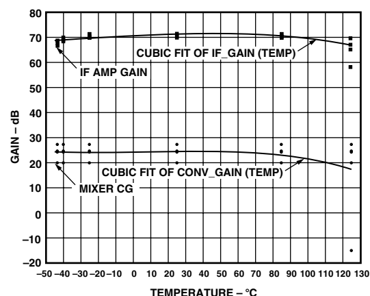
Figure 17. Mixer Conversion Gain and IF Amplifier Gain vs. Temperature, V_{\text{POS}} = 3\text{ V} , V_{\text{GAIN}} = 0.3\text{ V} , V_{\text{REF}} = 1.5\text{ V} , \text{IF} = 10.7\text{ MHz} , \text{RF} = 250\text{ MHz}
