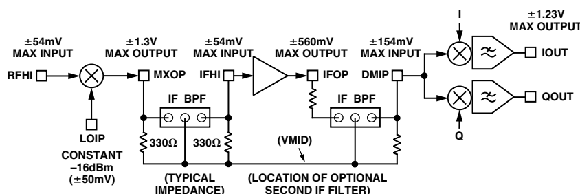
Figure 41. Signal Levels for Minimum and Maximum Gain
