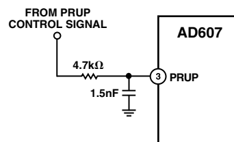
Figure 44. Proper Configuration of AD607 PRUP Signal
