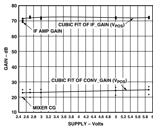
Figure 18. Mixer Conversion Gain and IF Amplifier Gain vs. Supply Voltage, T = 25^{\circ}\text{C} , V_{\text{GAIN}} = 0.3\text{ V} , V_{\text{REF}} = 1.5\text{ V} , \text{IF} = 10.7\text{ MHz} , \text{RF} = 250\text{ MHz}
