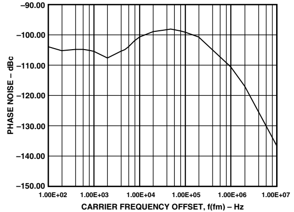
Figure 22. PLL Phase Noise L(F) vs. Frequency, V_{\text{POS}} = 3\text{ V} , C3 = 0.1\text{ }\mu\text{F} , \text{IF} = 10.7\text{ MHz}
