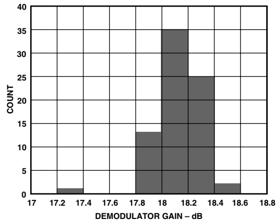
Figure 29. Demodulator Gain Histogram, T = 25^{\circ}\text{C} , V_{\text{POS}} = 3\text{ V} , \text{IF} = 10.7\text{ MHz}
