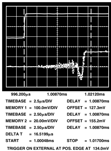
Figure 21. PLL Acquisition Time
