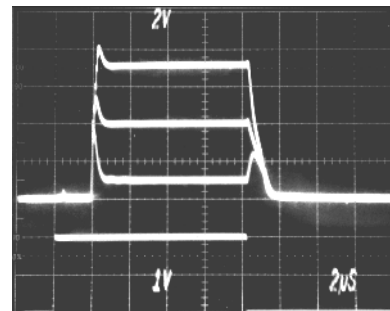
Figure 21. V_{LOG} Output for 10.7 MHz CW Input with PRUP Toggled ON and OFF; Top Trace: +5 dBm Input; Middle Trace: -35 dBm Input; Bottom Trace: -75 dBm; PRUP Input from HP8112A: 0 to 4 V, 10\ \mu\text{s} Pulsewidth with 10 kHz Repetition Rate
