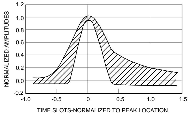
Figure 4. DSX-3 Isolated Pulse Template for Bellcore TR-NWT-000499
