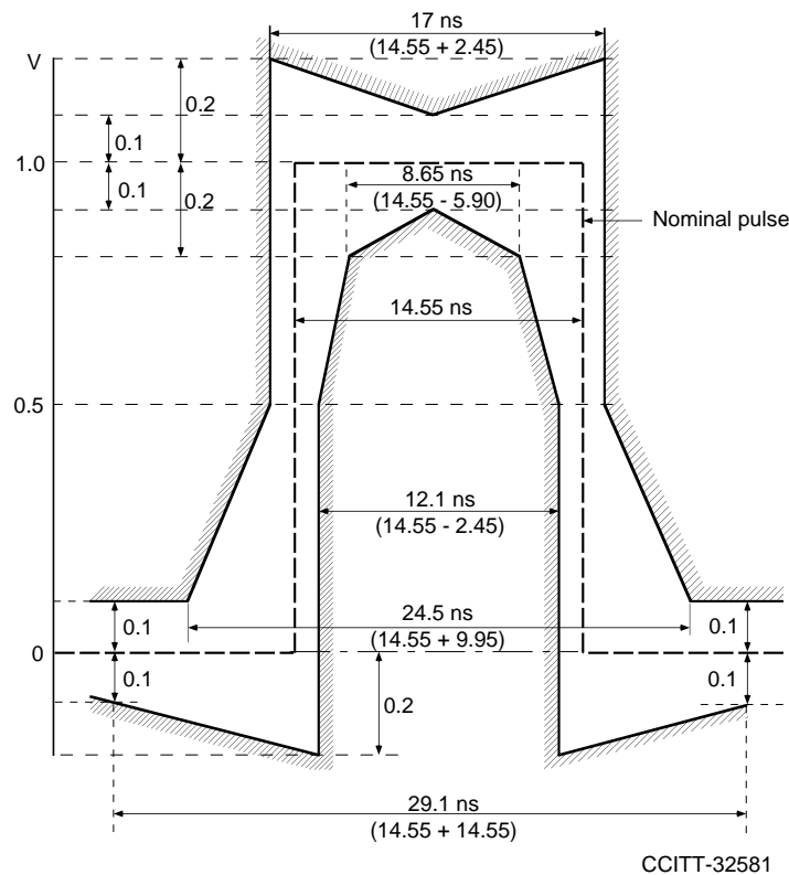
Figure 6. CCITT G.703 Pulse Mask at the 34,368-kbit/s Interface
