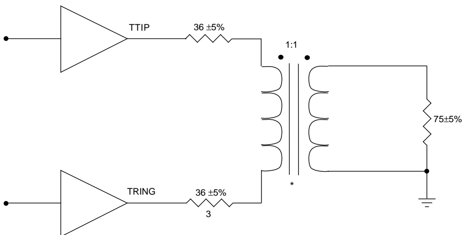
Figure 2. Transmit Pulse Amplitude Test Circuit
