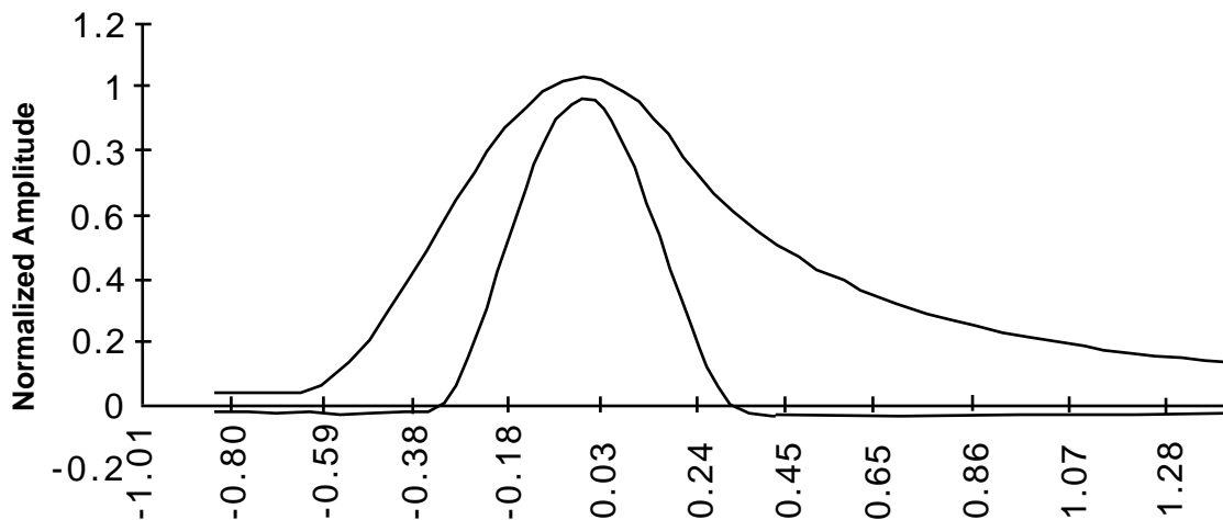
Figure 5. STSX-1 Isolated Pulse Template for Bellcore TA-TSY-000253
