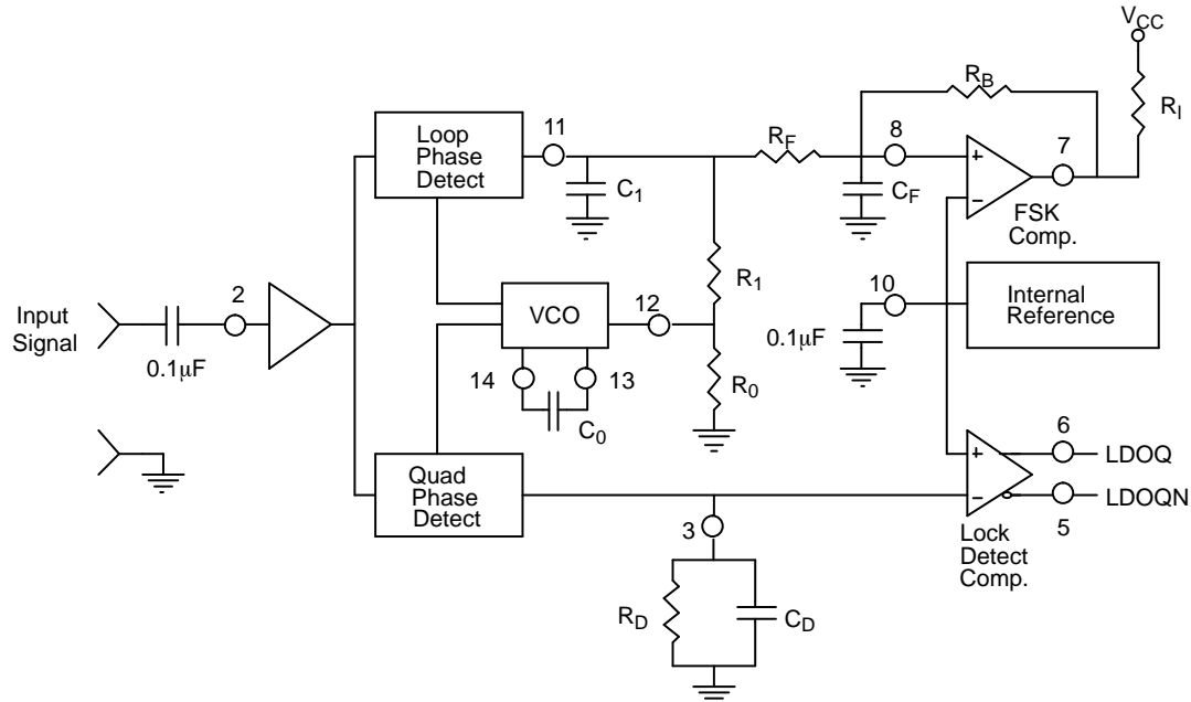
Figure 3. Generalized Circuit Connection for FSK and Tone Detection
