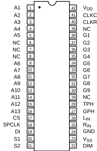
42 Lead SDIP (0.600")
