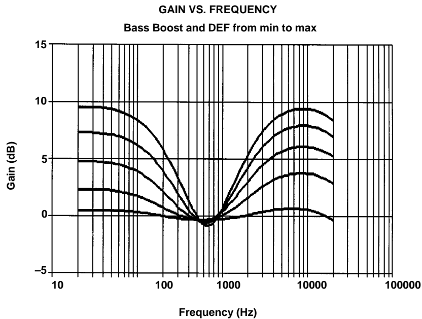
Figure 3. Gain Response
