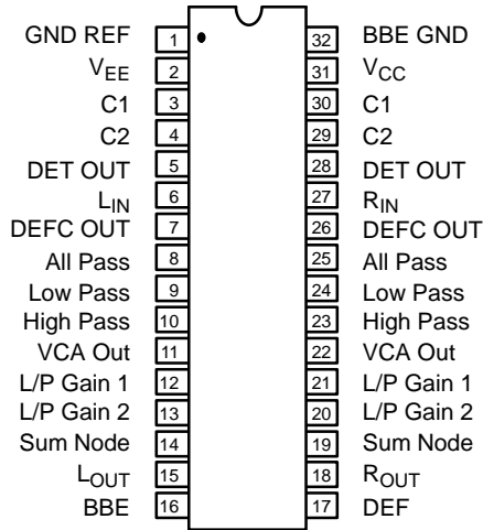
32 Lead SDIP (0.400\"
