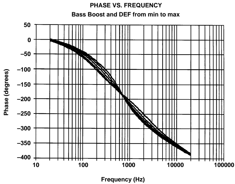
Figure 2. Phase Response
