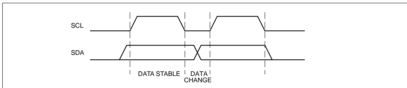
Figure 1. Data Validity
