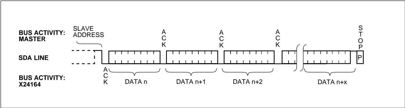
Figure 9. Sequential Read
