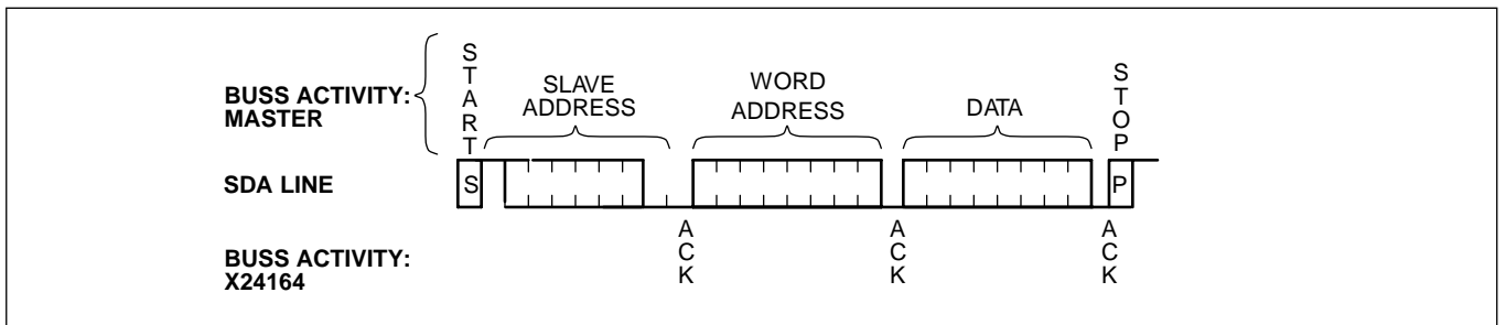
Figure 5. Byte Write
