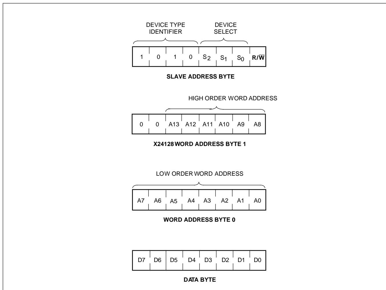
Figure 4. Device Addressing
