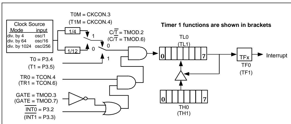
Figure 12: Timer/Counter Mode 2
