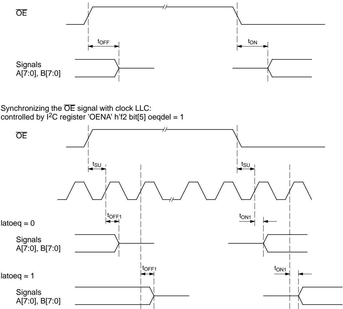
Fig. 5–4: Drive Control by \overline{OE} input
