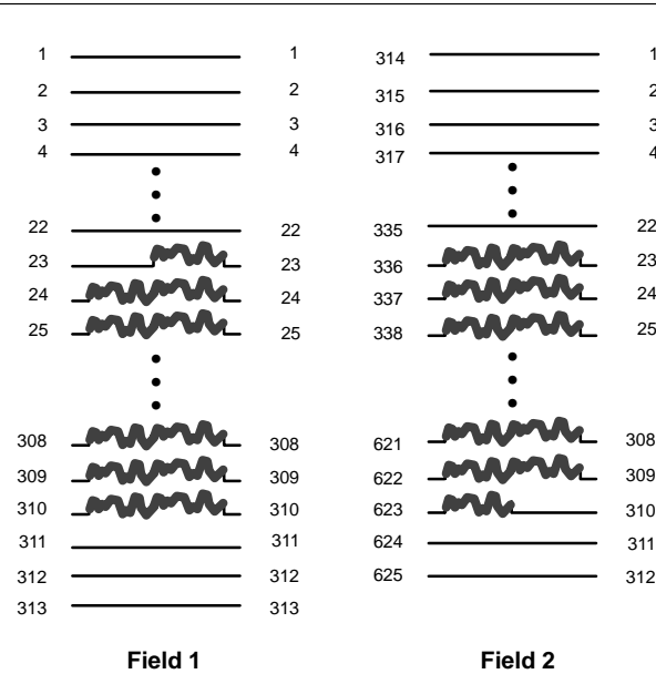
Fig. 2–34: Mapping for 625/50 line systems
