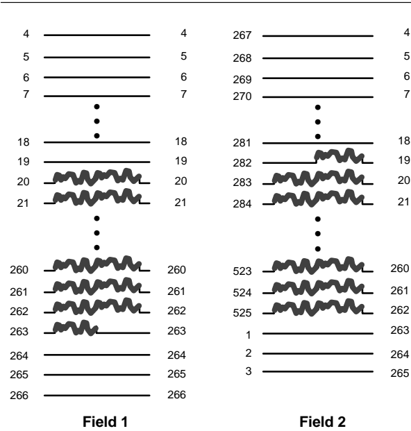
Fig. 2–33: Mapping for 525/60 line systems
