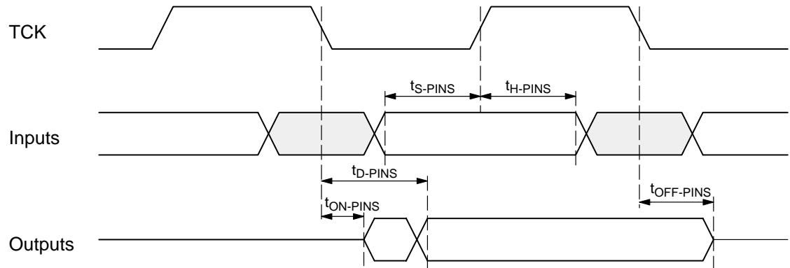
Fig. 5–6: Timing with respect to input and output signals
