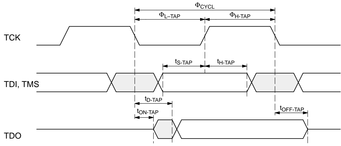
Fig. 5–5: Timing of Test Access Port TAP
