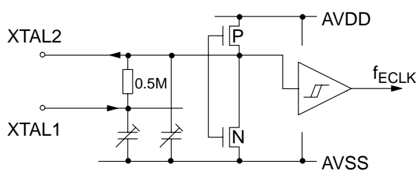
Fig. 3–8: Crystal Oscillator
