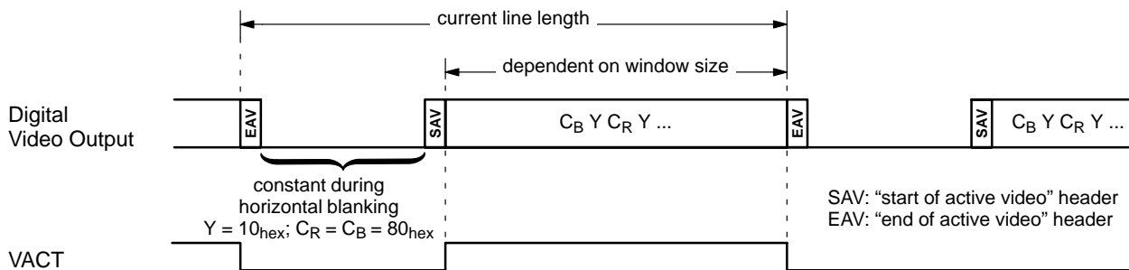
Fig. 2–18: Output of video or VBI data with embedded reference headers (according to ITU-R656)
