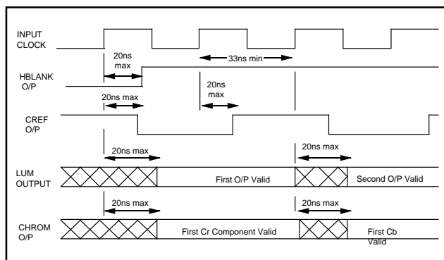
Fig 5 : Luminance and Chrominance Output Timing
