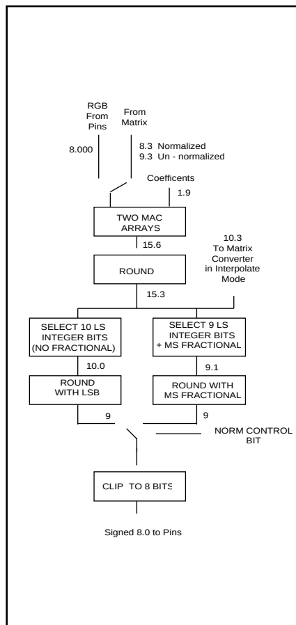
Figure 4. Bit significance
