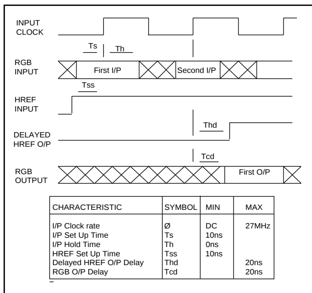
Figure 6. RGB I/O Timing (Advanced Data)
