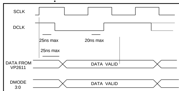
Figure 2. DBUS Timing
