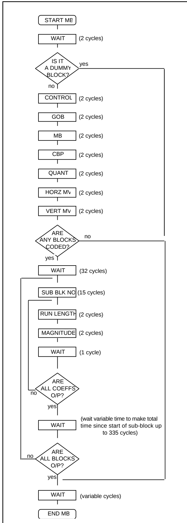
Fig 3 : DBUS Port Flow Chart
