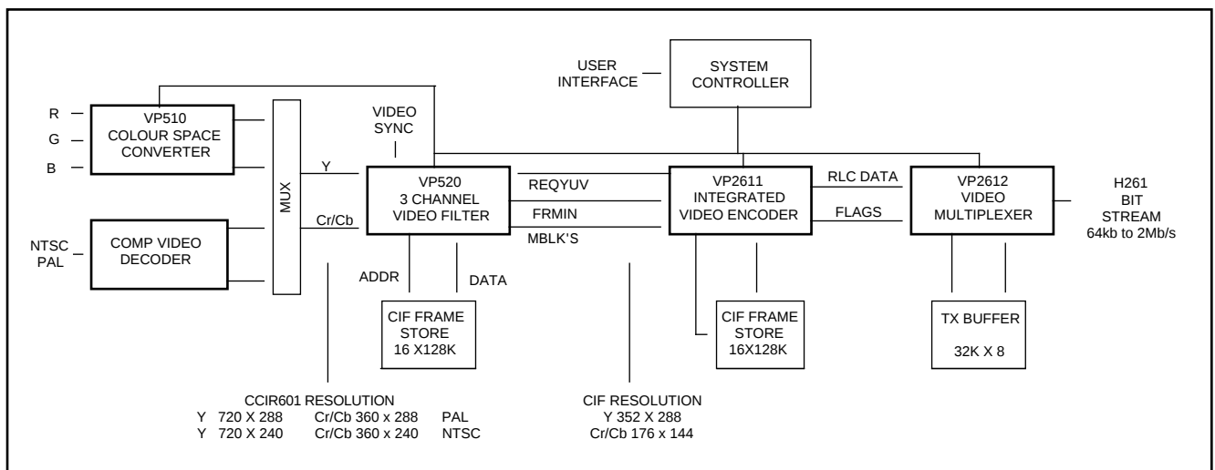
Fig 1 : Typical Video Conferencing Transmission System
