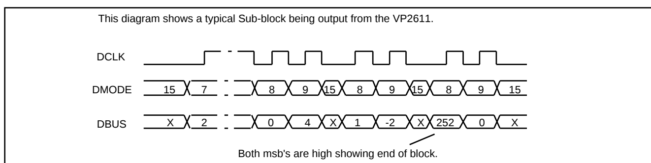
Fig 9: DBUS Timing
