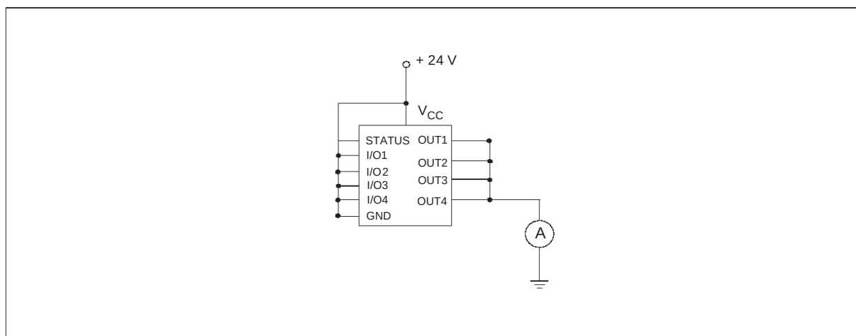
Fig. 3: I_{LGND} Test Configuration
