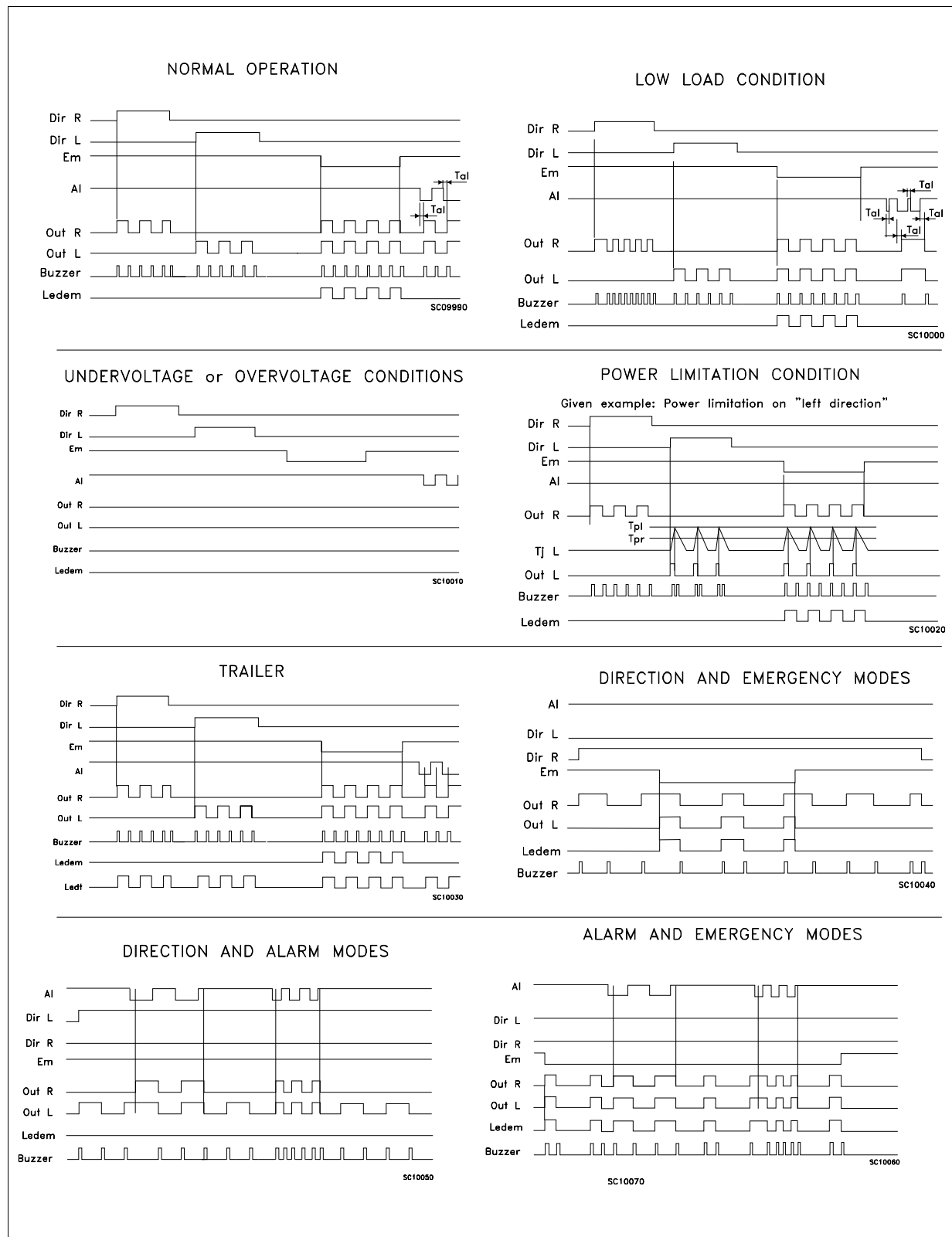
FIGURE 2: Switching Waveforms
