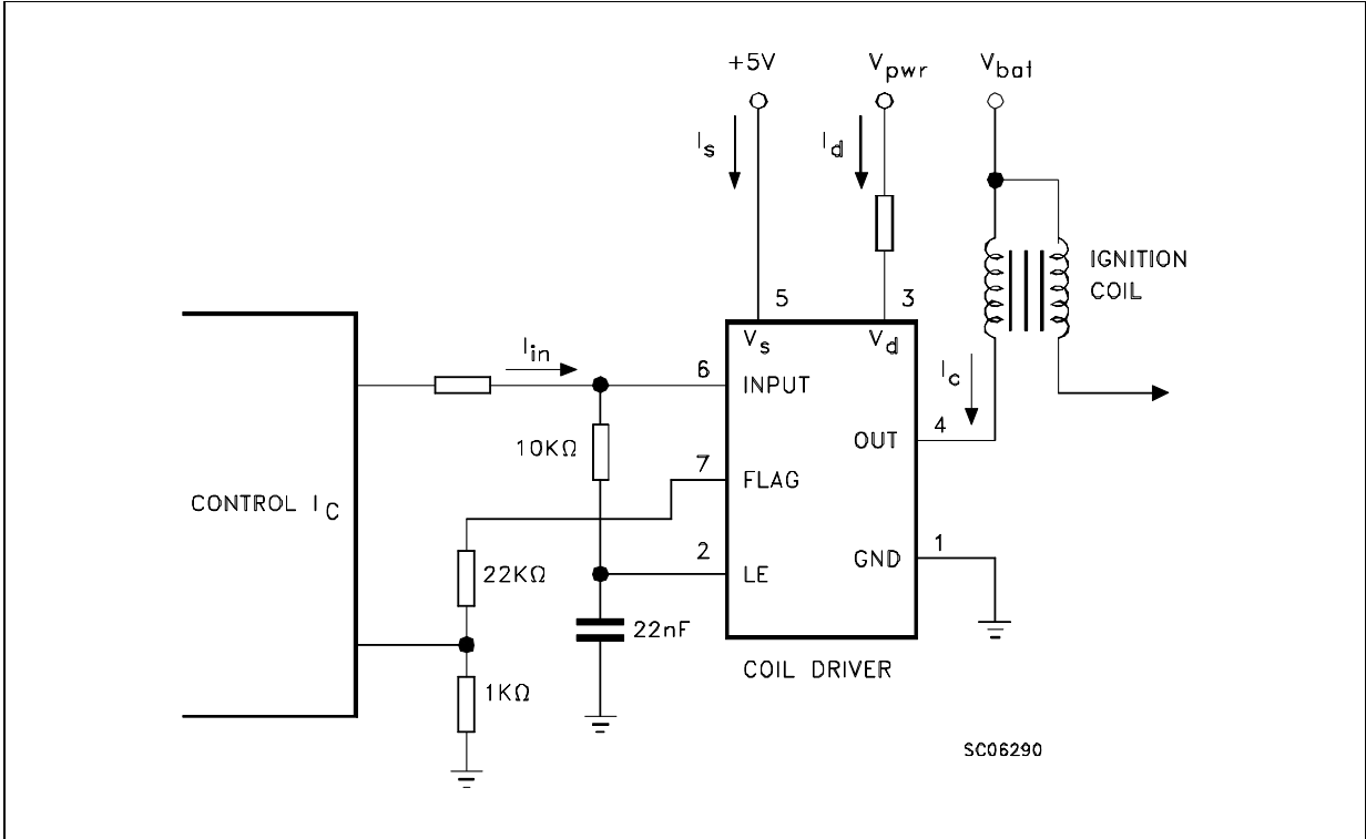
FIGURE1: Application Circuit
