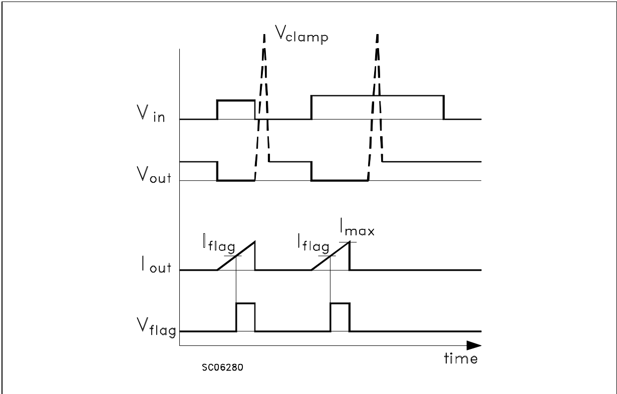
FIGURE2: Switching Waveforms
