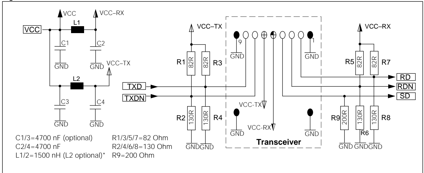
Figure 1. Schematic
