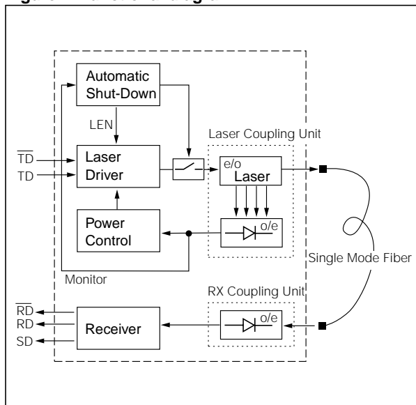
Figure 1. Functional diagram
