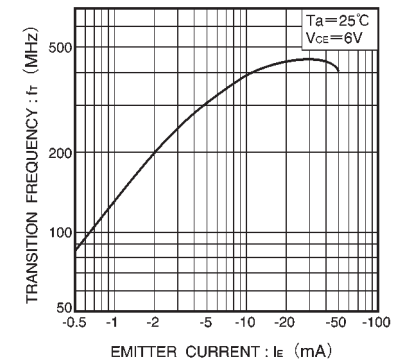
Fig.18 Gain bandwidth product vs. emitter current
