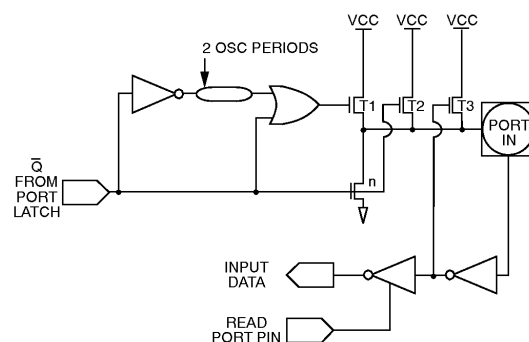
Figure 4. I/O Buffers in the TSC80CL51 (Ports 1, 2, 3).
