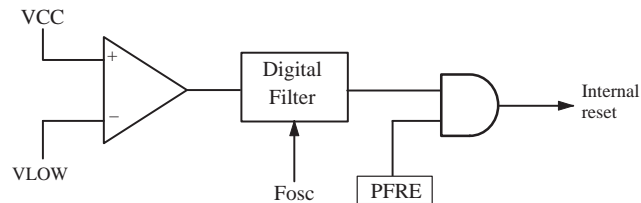
Figure 10 Power Fail Reset block diagram
