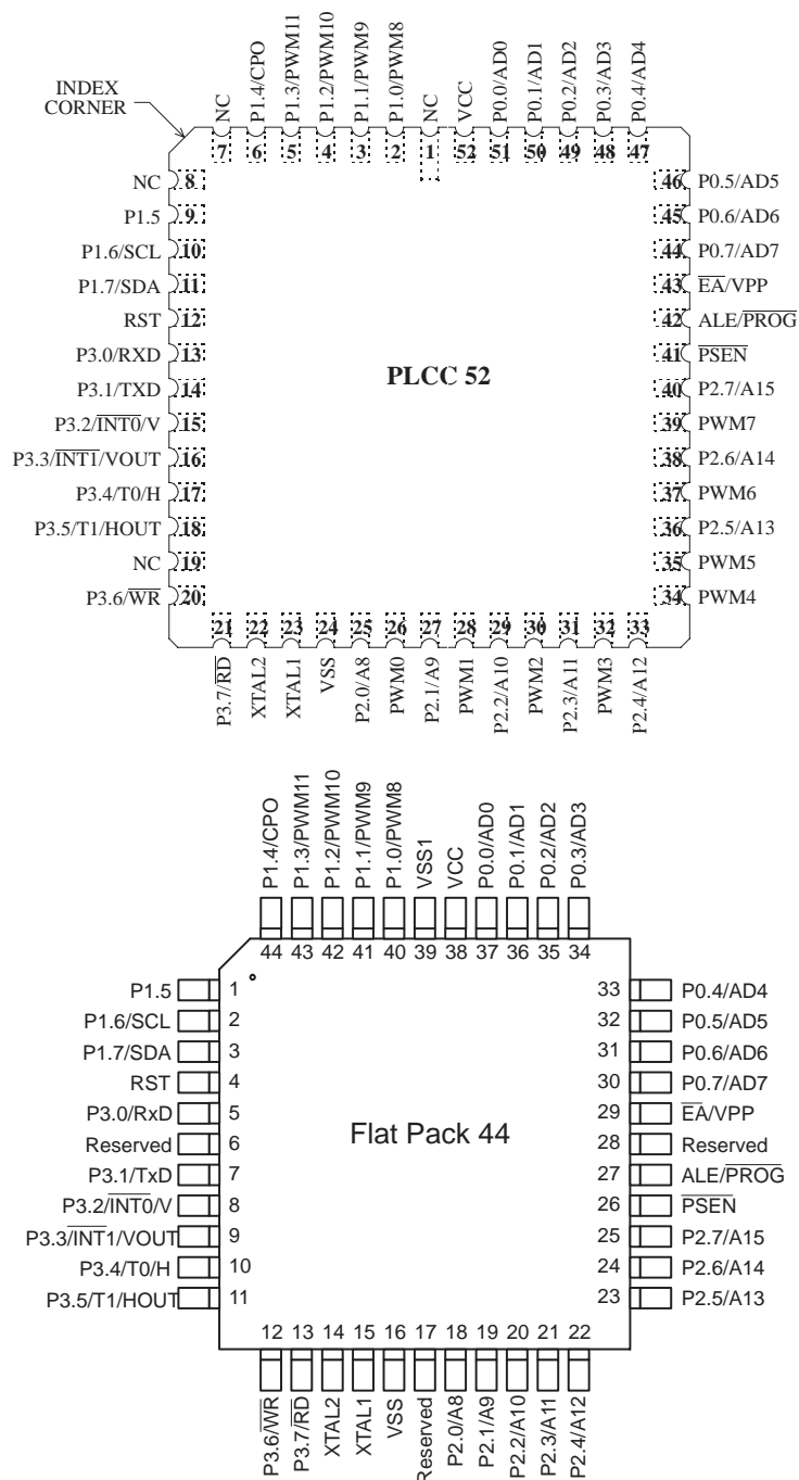
Figure 2 TSC8051i2 pin configurations
