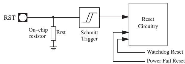
Figure 5 On-Chip Reset Configuration
