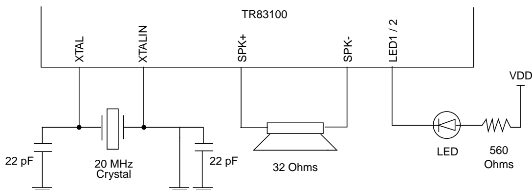
Figure 5 • Crystal, Speaker & LED connections
