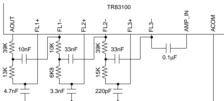
Figure 4 • Active Filter Connections
