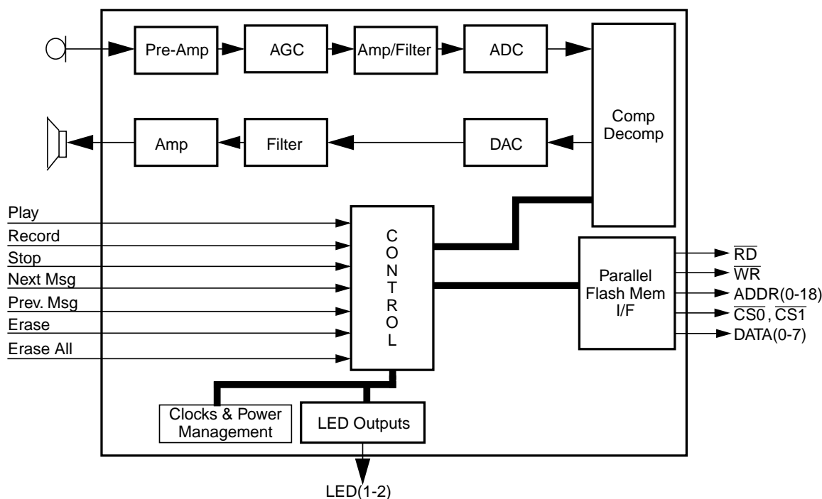
Figure 1 • TR83100 Voice Storage Controller
