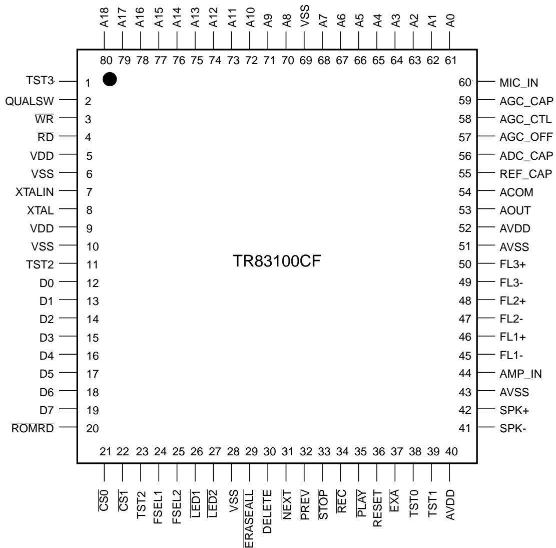
Figure 2 • Package Pin Layout, Top View
