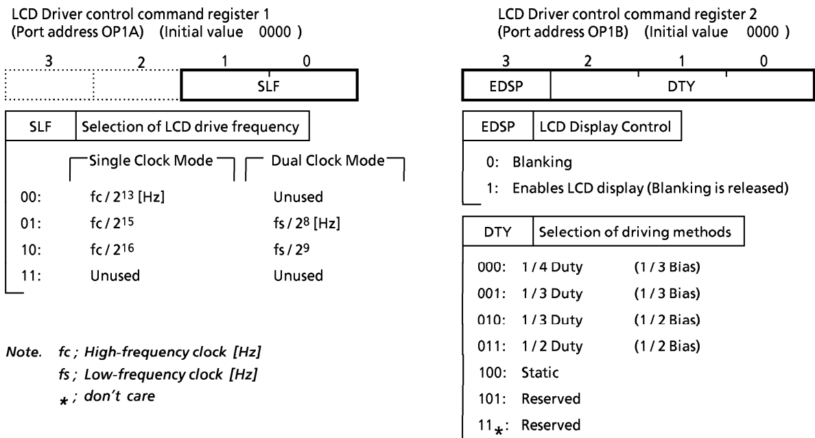
Figure 3-7. LCD Driver control Command Register
