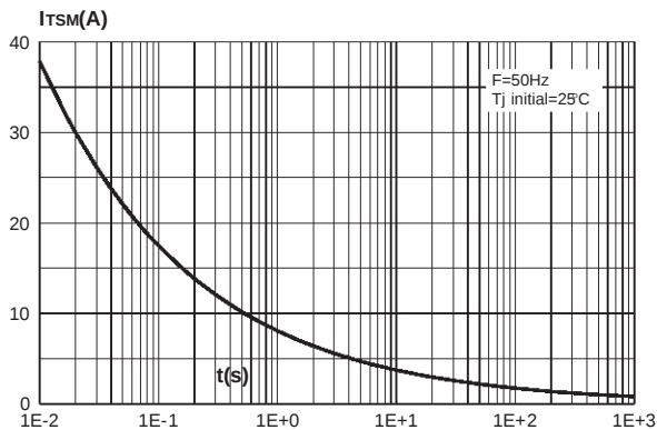
Fig. 5: Surge peak current versus overload duration (THDT58S).
