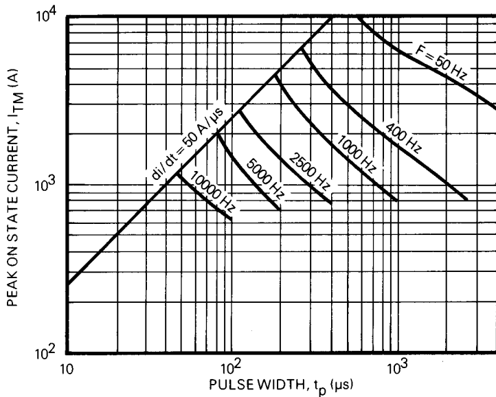
FIG.13 MAXIMUM ALLOWABLE PEAK ON-STATE CURRENT vs PULSE WIDTH FOR T_c = 65^\circ\text{C}
