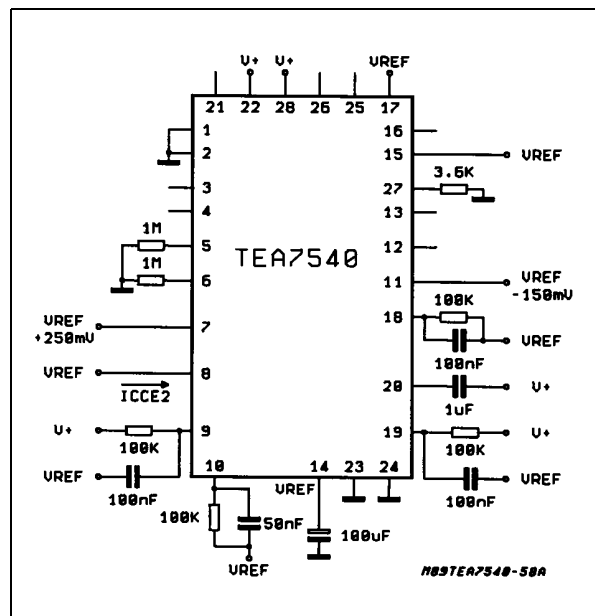
Figure 6: Test Configuration
