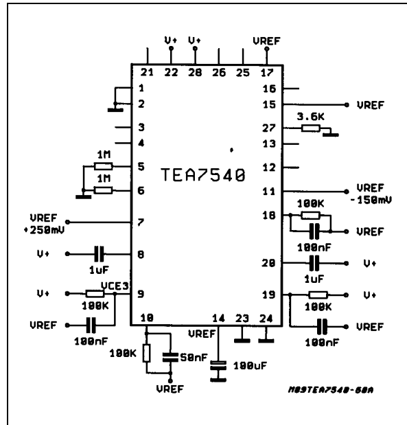
Figure 8: Test Configuration
