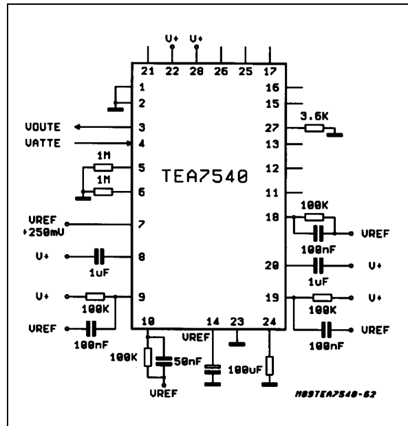
Figure 10: Test Configuration
