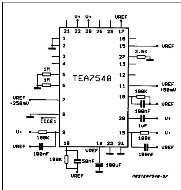
Figure 5: Test Configuration
