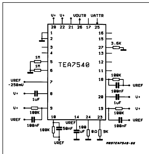
Figure 14: Test Configuration
