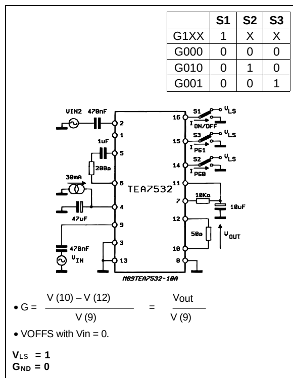
Figure 8 : Loudspeaker Amplifier : Gain/Distortion/Output Offset.
