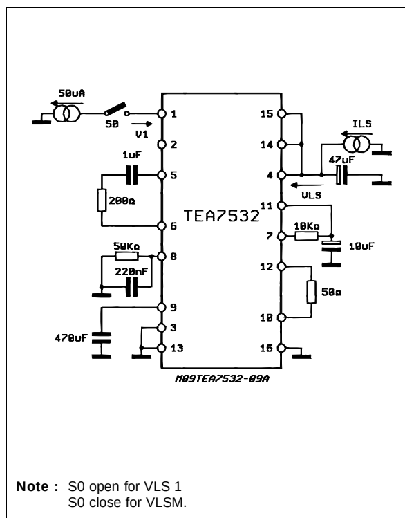
Figure 7 : Shuntvoltage Regulator/ Reference Voltage at Pin 1.
