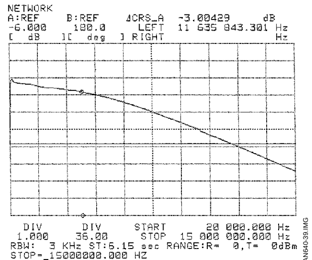
Figure 39 : LP Channel - Z = 100Ω
