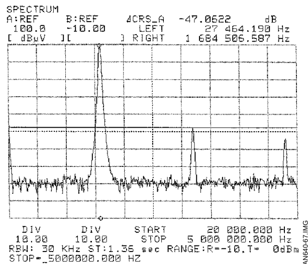
Figure 67 : I_{REC} = 60\text{mA p-pk}
