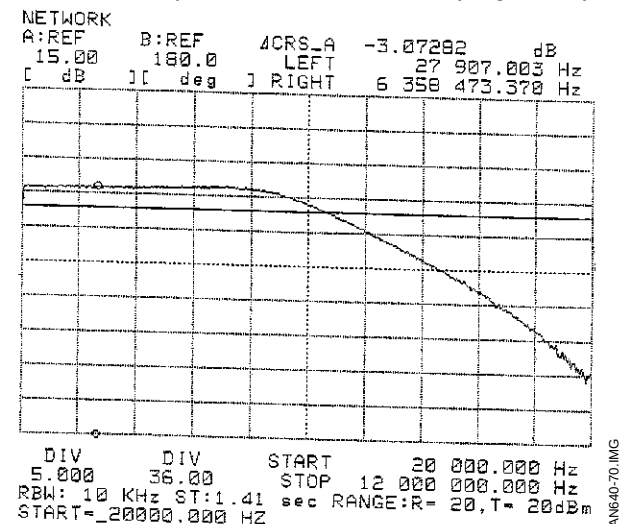
Figure 70 : Z = \text{VTR drum} , I_{REC} = 20\text{mA p-pk} ( R_{105} = 330\Omega in the damping circuit)
