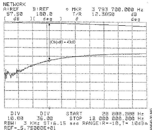
Figure 30 : H2SP - R_{IN} = \infty (open)
