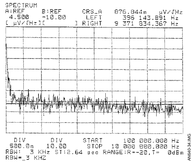
Figure 34 : I_N ( e_N = \frac{V_{OUT}}{G_V \cdot Z_{IN}} , Z_{IN} = 500\Omega ) I_N = 1.88\text{pA}/\sqrt{\text{Hz}}
