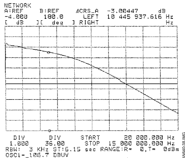
Figure 38 : SP Channel - Z = 100Ω
