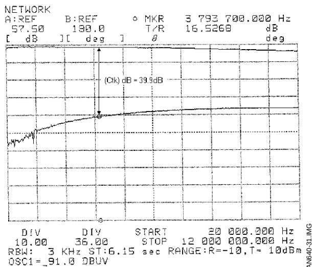
Figure 31 : H1SP - R_{IN} = \infty (open)
