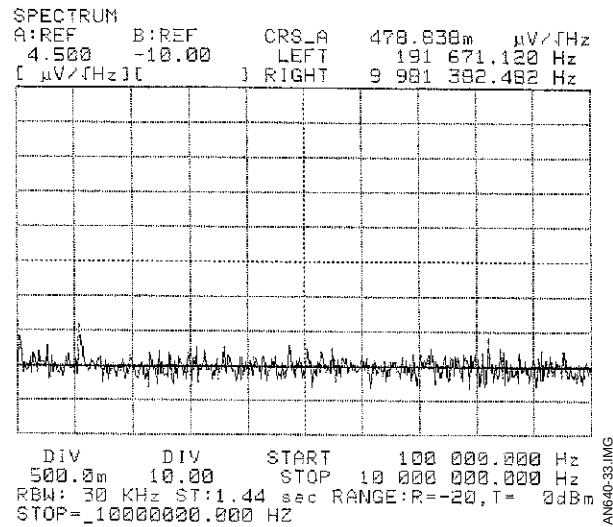
Figure 33 : e_N ( e_N = \frac{V_{OUT}}{G_V} , G_V = 59.3\text{dB} ) e_N = 0.58\text{nV}/\sqrt{\text{Hz}}
