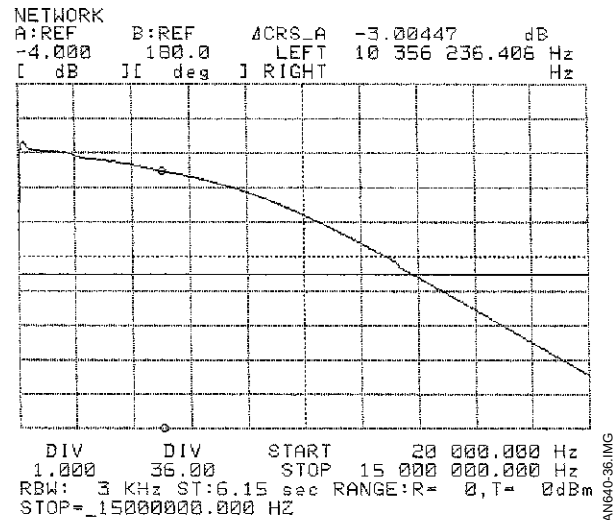
Figure 36 : SP Channel - Z = 100Ω
