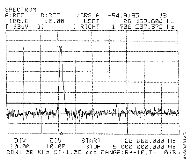
Figure 68 : I_{REC} = 10\text{mA p-pk}
