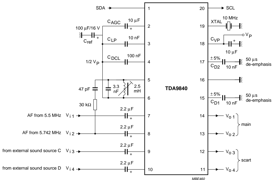
Fig.5 Test circuit of the stereo decoder TDA9840.
