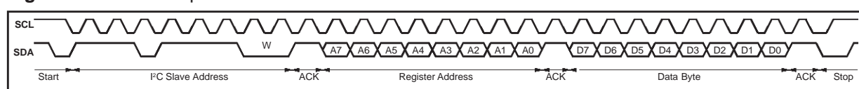
Figure 6 : I 2 C Write Operation
