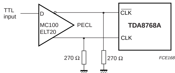
Fig 18. Application diagram for Differential Clock input PECL compatible using a TTL to PECL translator.
