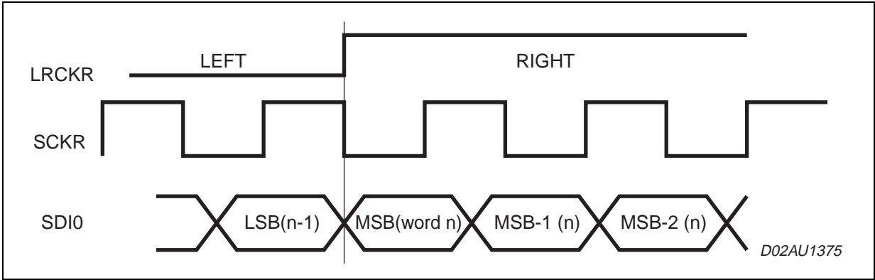
Figure 6. SAI protocol when RLRS=0; RREL=1; RCKP=1; RDIR=0
