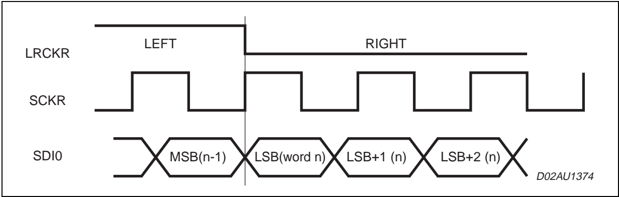
Figure 5. SAI protocol when RLRS=0; RREL=0; RCKP=0; RDIR=0
