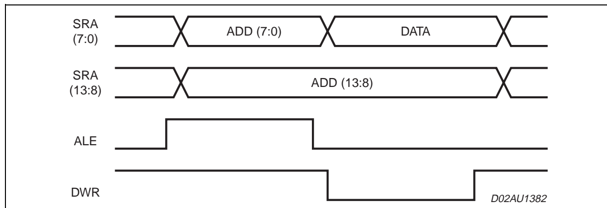
Figure 17. External Memory Interface SRAM Write Cycle
