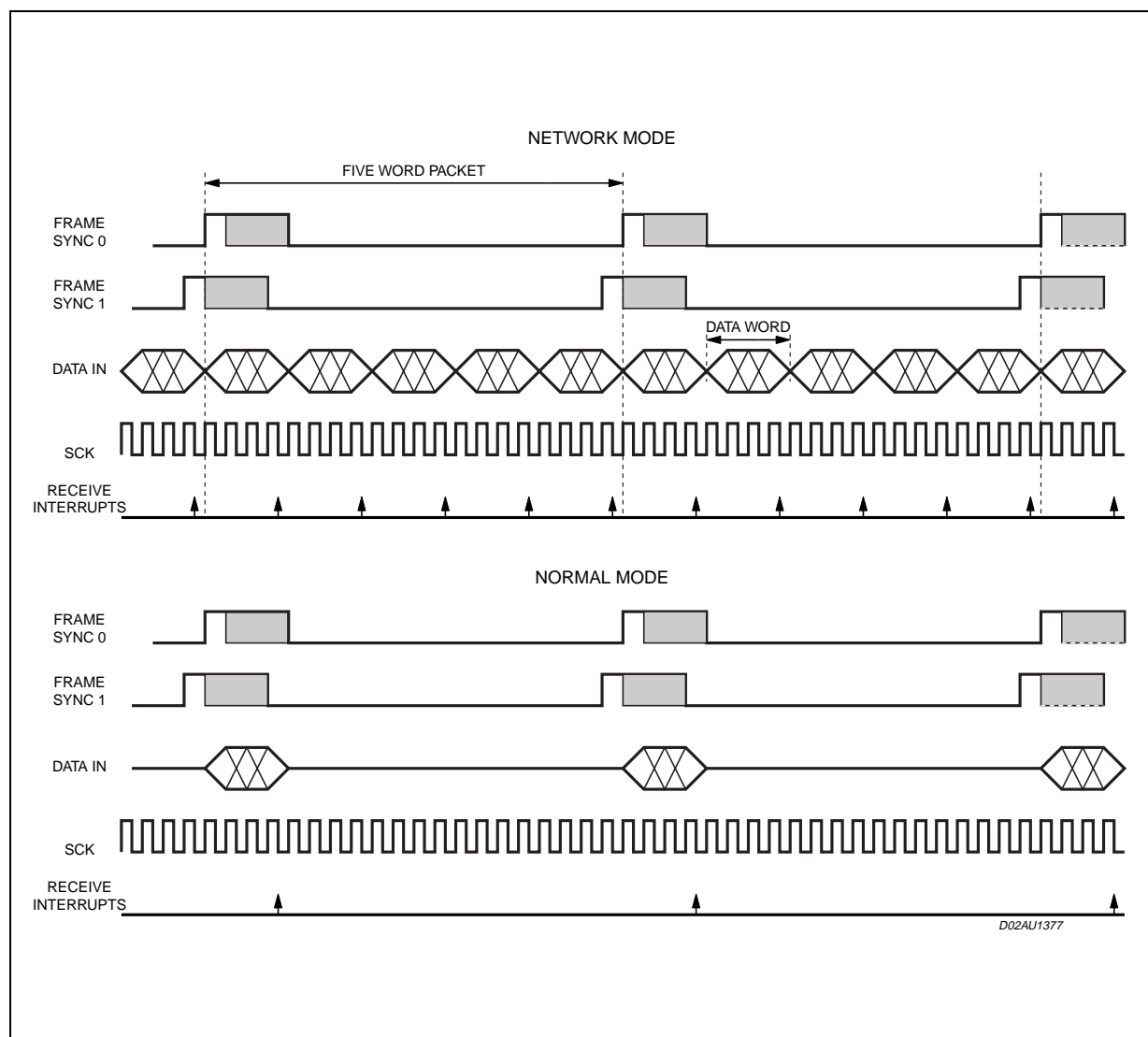
Figure 7. SSI Protocol
