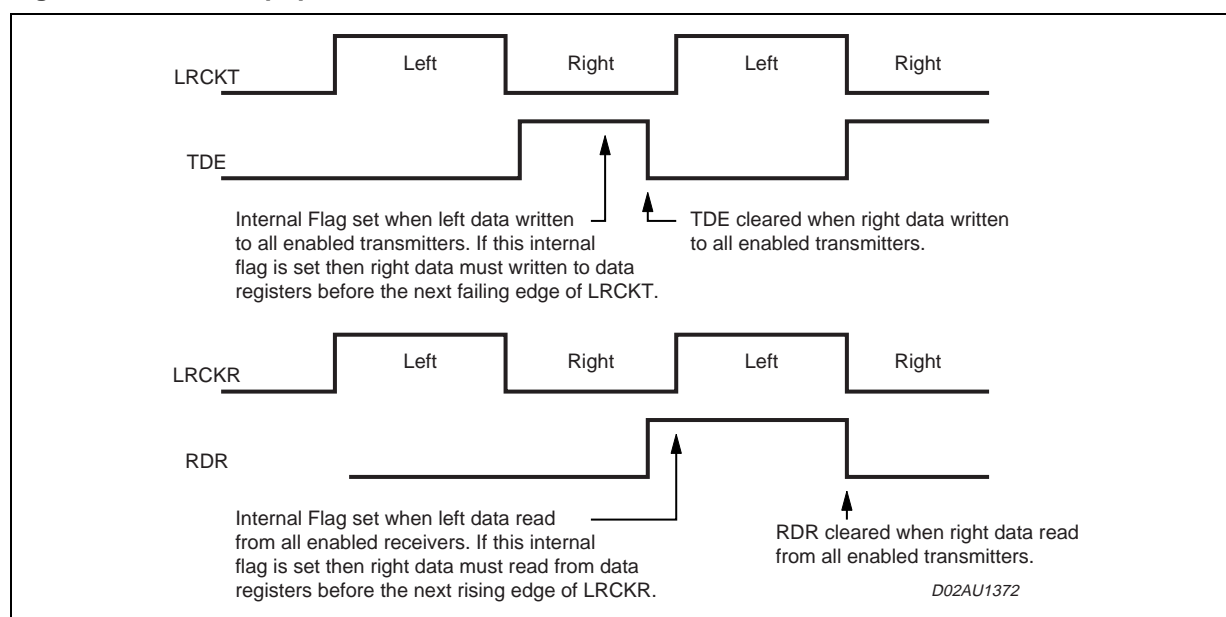
Figure 2. SAI Interrupt protocol
