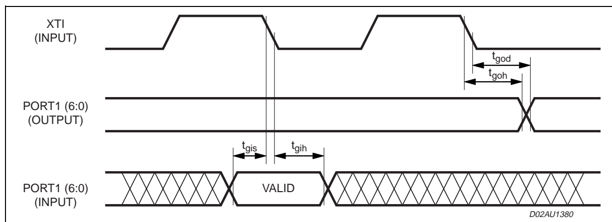
Figure 10. GPIO Timing
