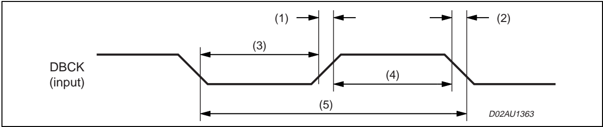
Figure 12. Debug Port Acknowledge Timing
