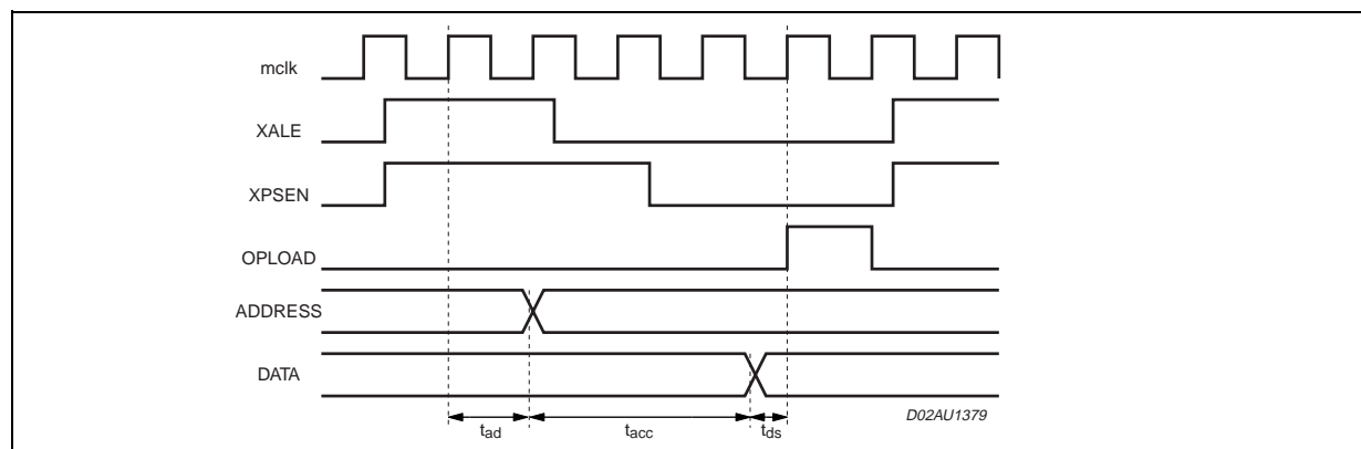
Figure 9. Timing diagram for External Memory Interface
