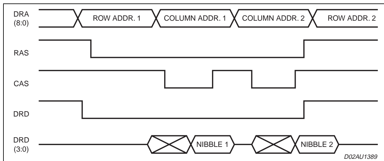
Figure 19. DRAM Write Cycle
