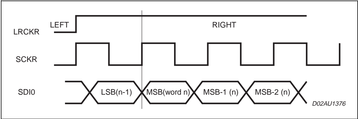
Figure 6. SAI protocol when RLRS=0; RREL=1; RCKP=1; RDIR=0
