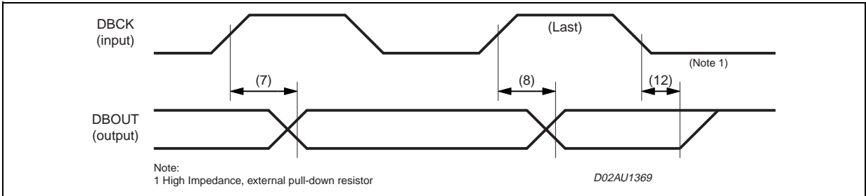
Figure 15. Debug Port DBCK Next Command After Read Register Timing
