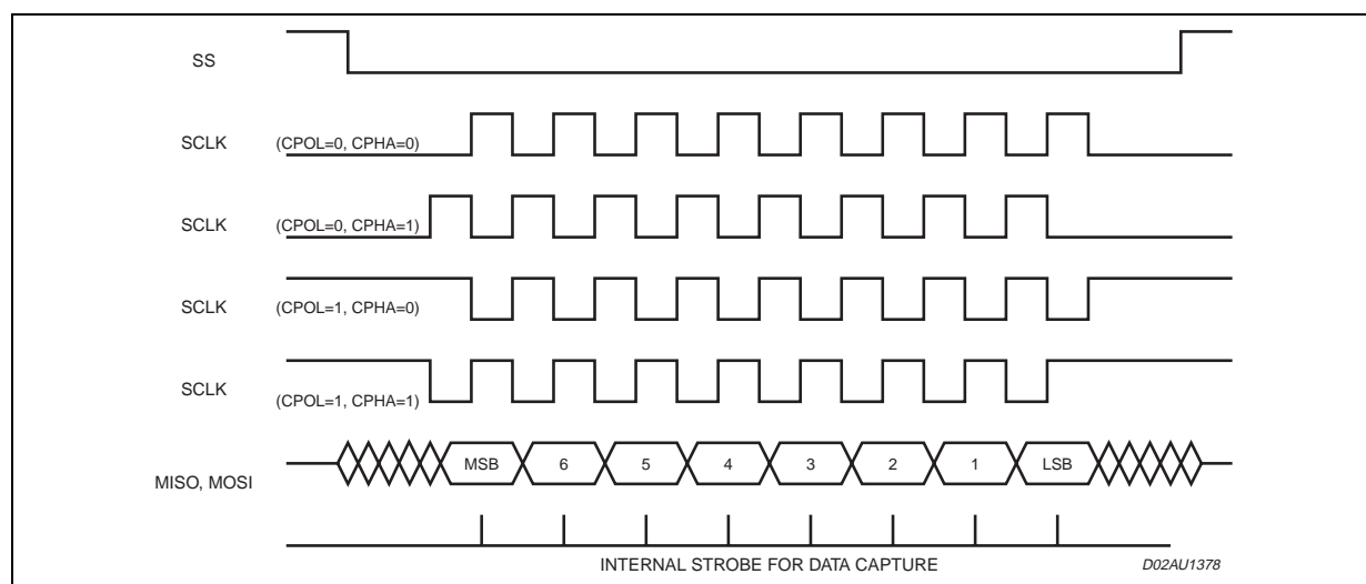
Figure 8. SPI Clocking scheme
