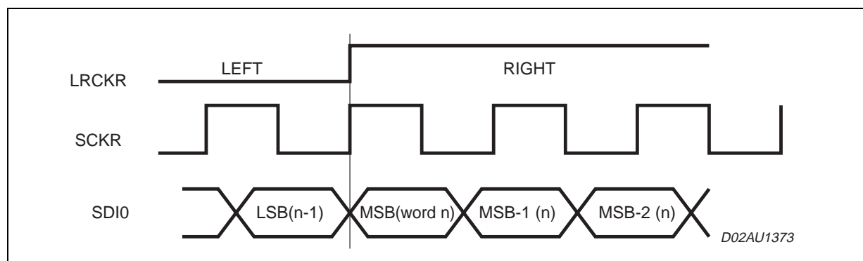
Figure 3. SAI protocol when RLR=0; RREL=0; RCKP=1; RDIR=0.
