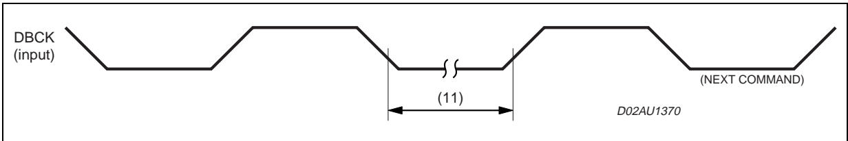
Figure 15. Debug Port DBCK Next Command After Read Register Timing
