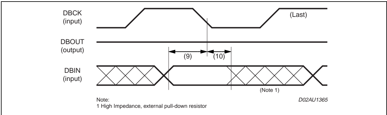
Figure 14. Debug Port Read Timing
