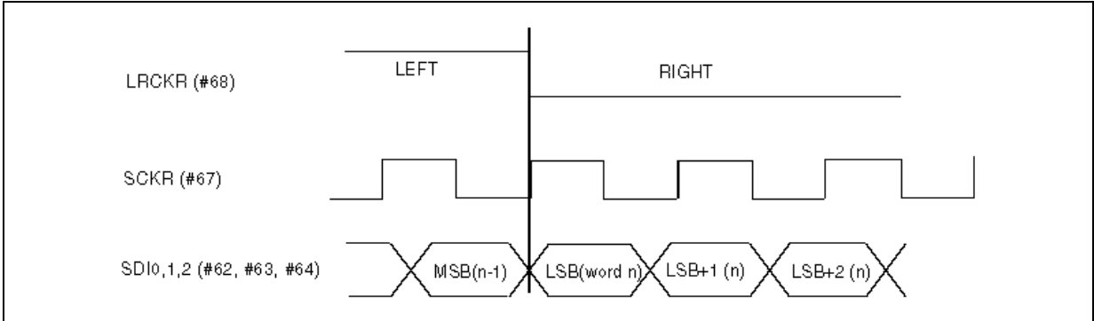
Figure 4. SAI protocol when RLRS=0; RREL=0; RCKP=0; RDIR=0.
