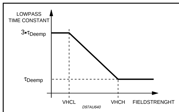
Figure 21. Highcut characteristics
