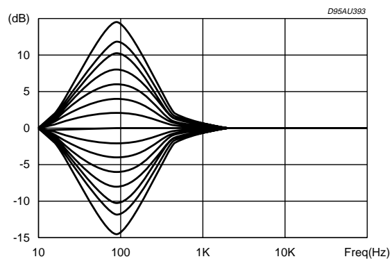
Figure 20: Loudness
