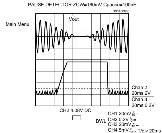
Figure 17: Pause Detector
