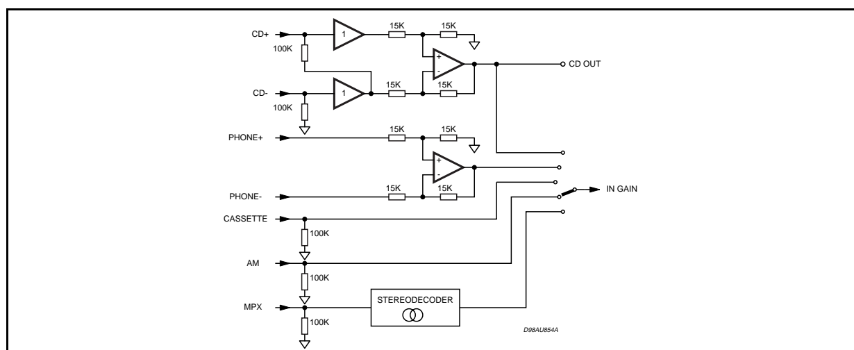
Figure 4. Input stages
