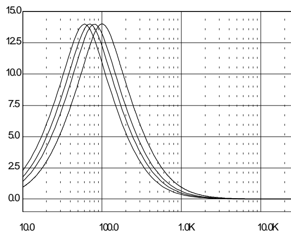
Figure 9. Bass normal and DC Mode @ Gain = 14dB, f_c = 80\text{Hz}
