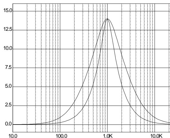
Figure 12. Mid Q-factor @ f_c=1\text{kHz} , Gain=14dB
