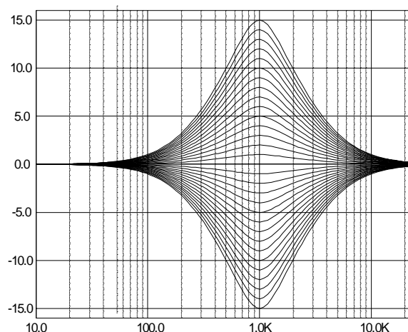
Figure 10. Mid Control @ f_c=1\text{kHz} , Q=1
