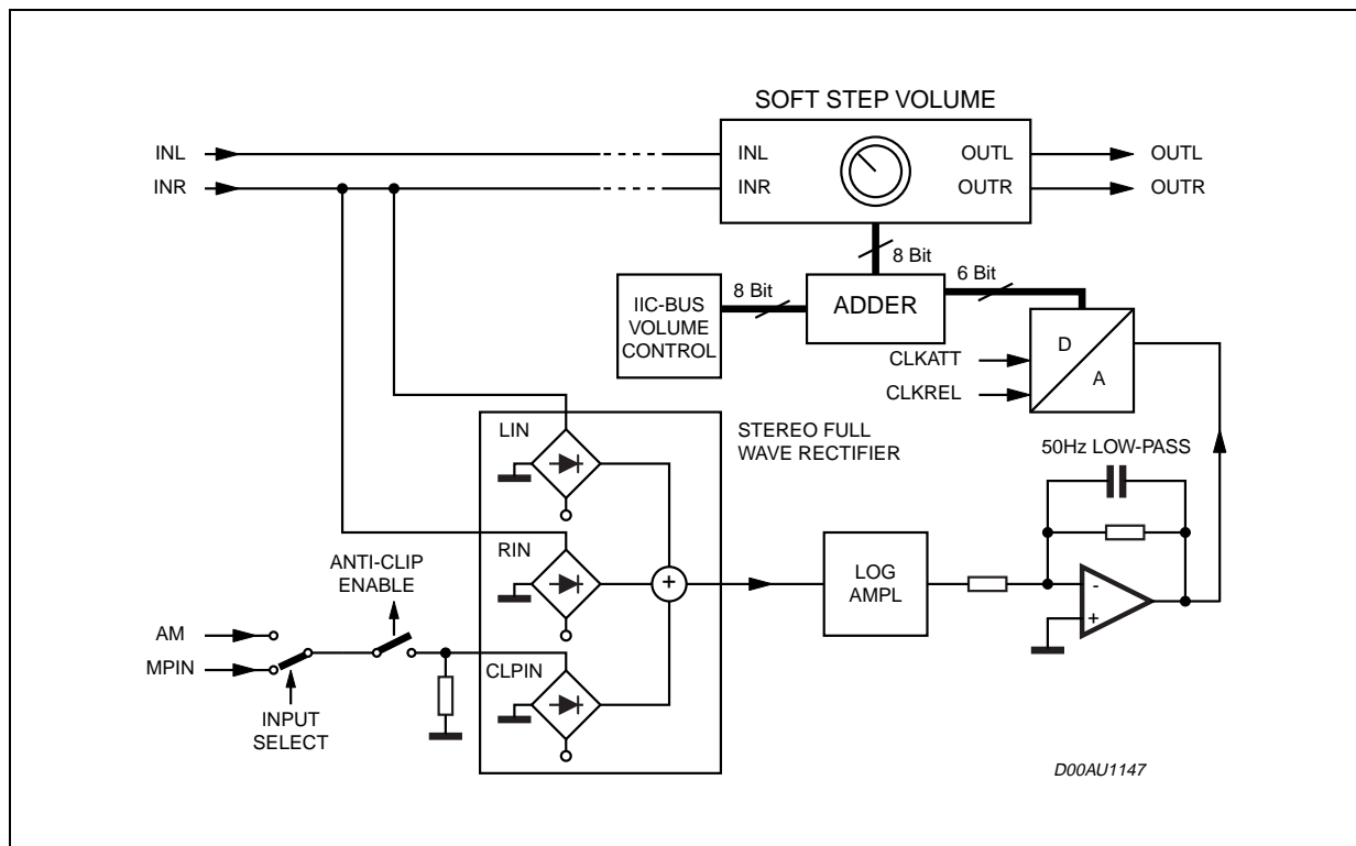
Figure 15. Comander Block Diagram
