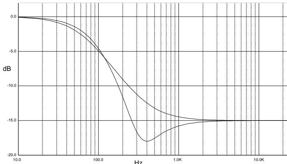
Figure 4. 1st and 2nd Order Loudness @ Attn. = 15dB, f_p=400\text{Hz}
