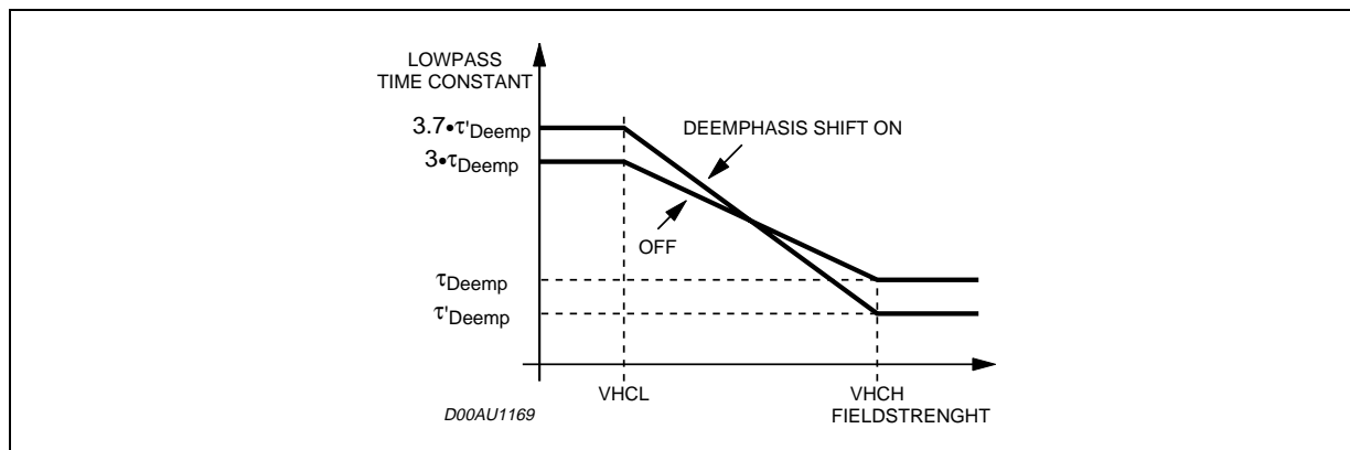
Figure 30. Highcut characteristics
