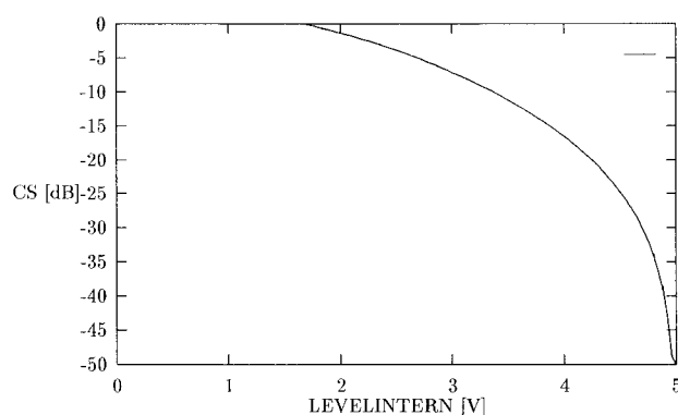
Figure 28. Internal stereoblend characteristics
