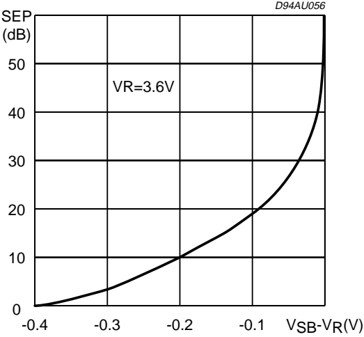
Figure 2: Stereo Blend
