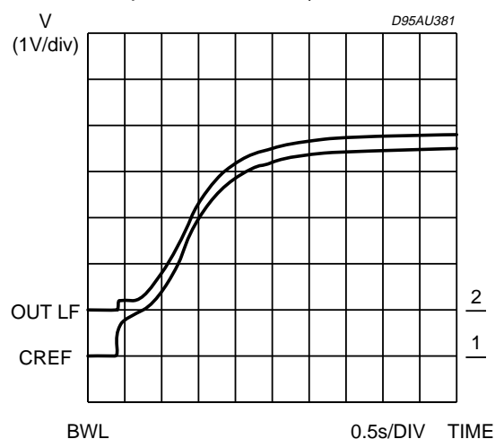
Figure 9: Power on Time Constant vs Cref Capacitor C REF = 10μF
