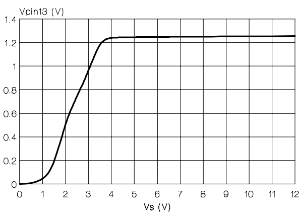
Figure 36: D.C. Voltage pin 13 vs. Supply Voltage
