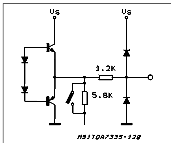
Figure 11: PINS: 5 - 24
