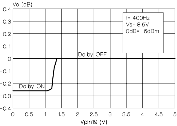
Figure 40: Load Characteristics
