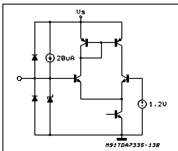
Figure 12: PINS: 7
