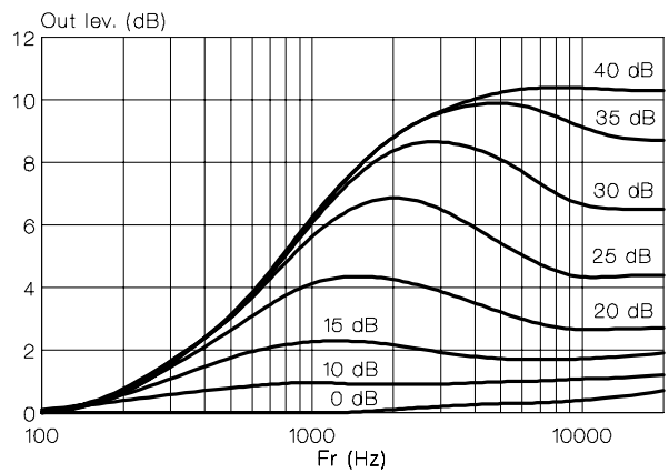
Figure 50: Dolby-B Table
