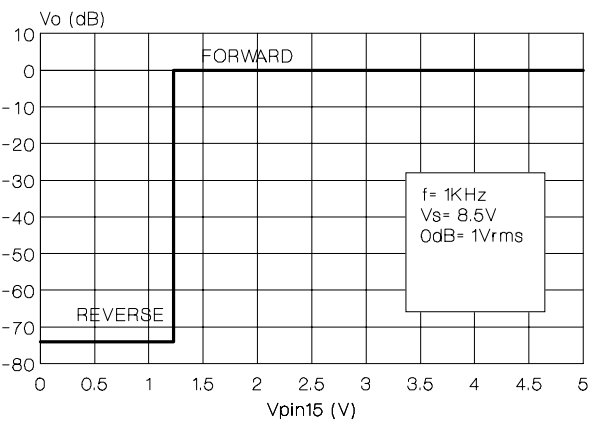
Figure 40: Load Characteristics
