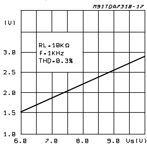
Figure 11: Output Clipping Level vs. Supply Voltage
