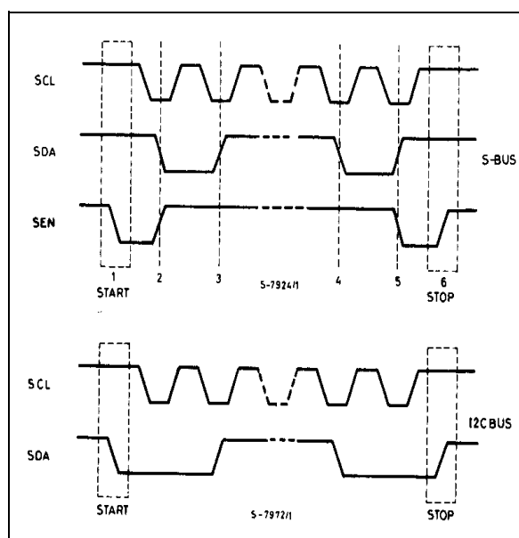
Figure 16: Timing Diagram of S-BUS and I 2 C BUS
