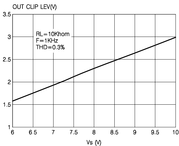
Figure 6: Output clip level vs. Supply Voltage.
