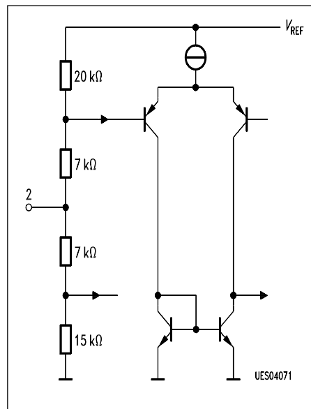
PATH (Pin 2)
