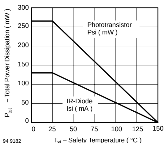
Figure 1. Derating diagram
