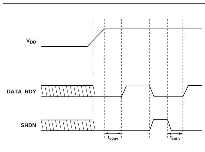
Figure 2. DATA_RDY, SHDN Operation Logic Diagram
