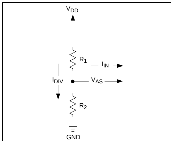
FIGURE 5-3: V AS CIRCUIT
