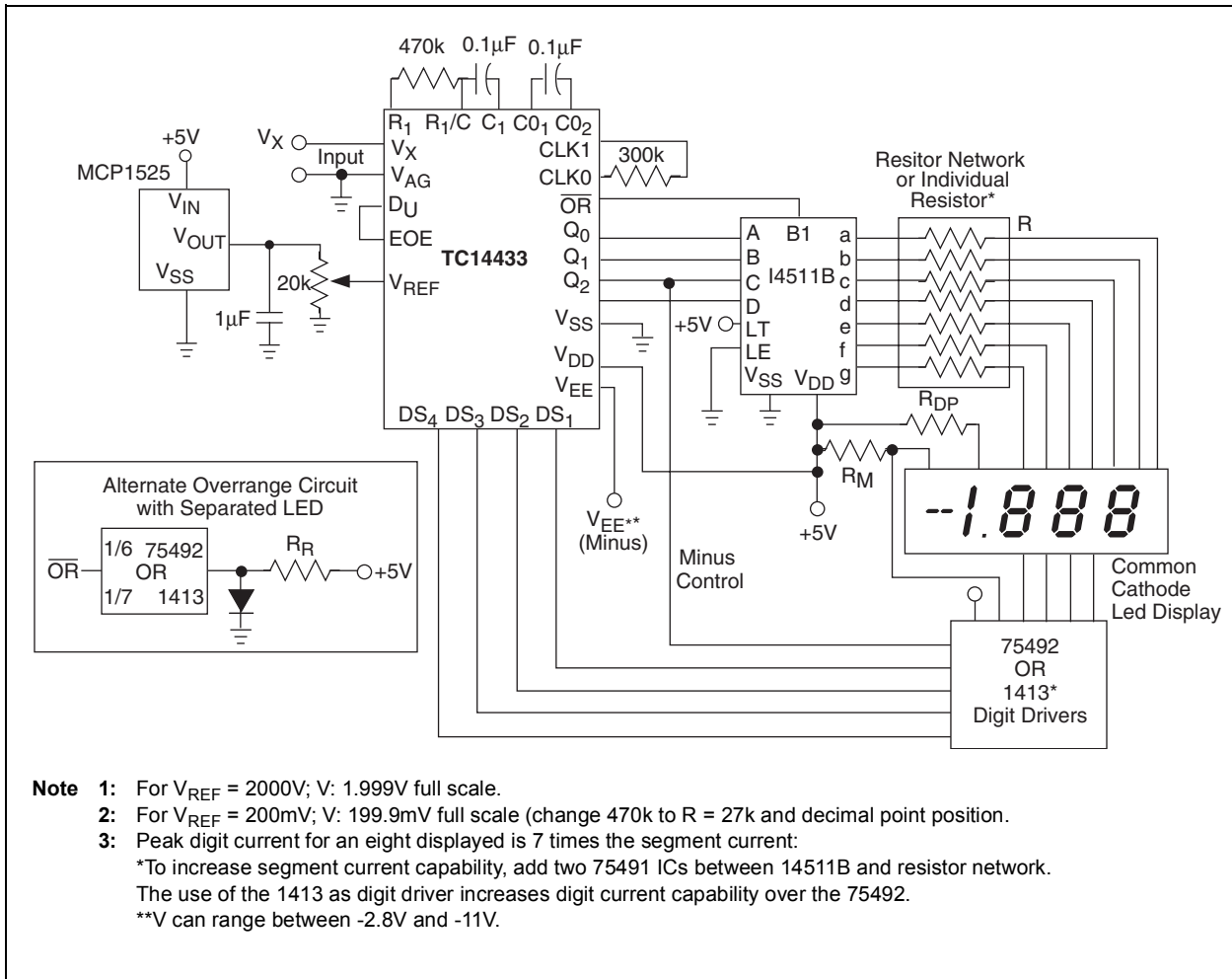
FIGURE 5-2: 3-1/2 DIGIT LED VOLTMETER WITH LOW COMPONENT COUNT USING COMMON CATHODE DISPLAYS
