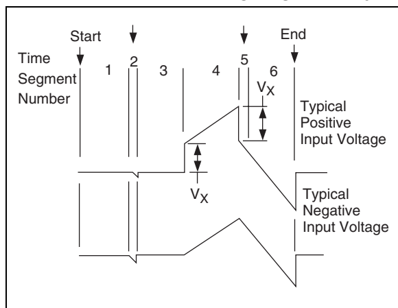
FIGURE 4-1: INTEGRATOR WAVEFORMS AT PIN 6
